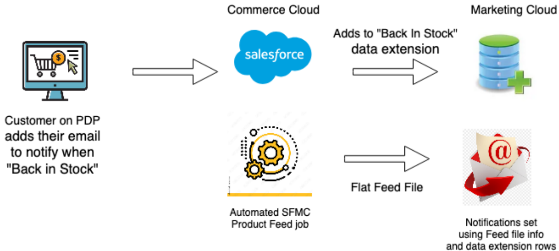
Data flows related to Back in Stock Notifications
